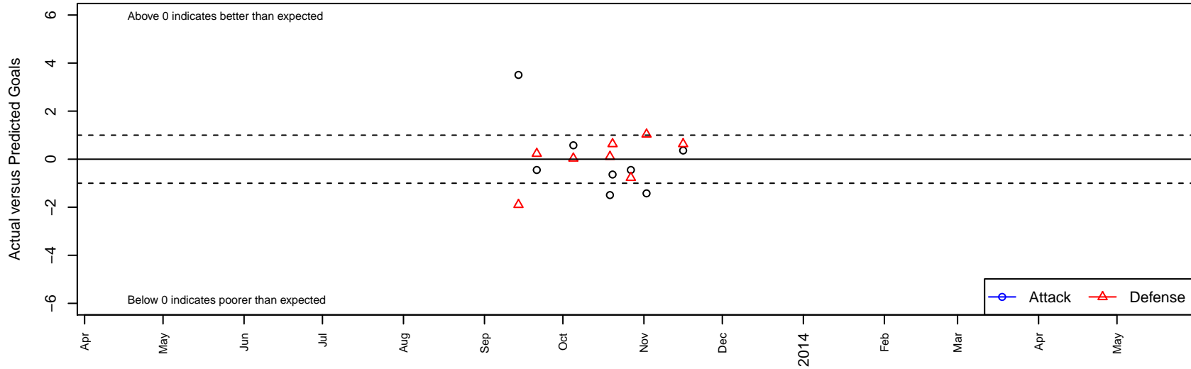
Novato United B02 Dots are actual minus expected GF (blue circles) and GA (red triangles). Blue line is smoothed change in attack strength. Red is smoothed change in defense strength.
